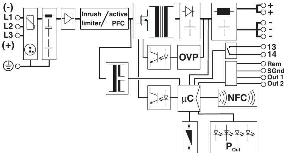
Figure 7 Block diagram
